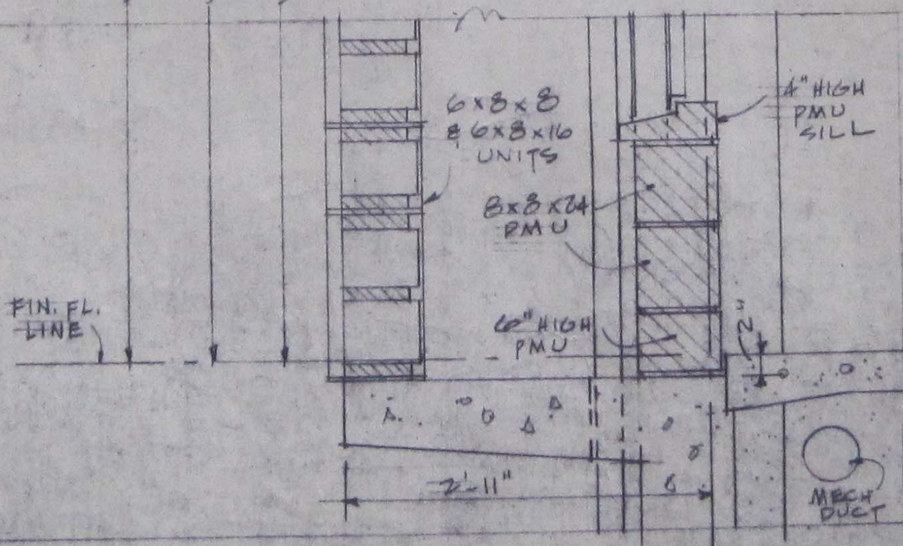
SECTION N \frac{3}{4}'' \text{ @ } 1'-0''
